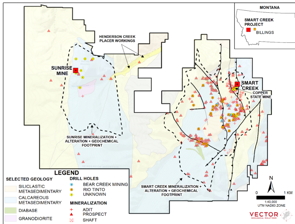
Figure 2. The economic geology of Smart Creek including surface geology, historical drilling, surface mineralization (adits, prospects and shafts) and anomalous footprints for the drill ready Smart Creek and Sunrise targets.
